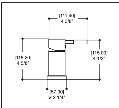
THERMOSTATIC MIXER
