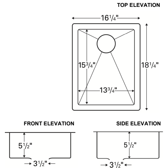
Edge Series Sink Installed in Solid Surface
