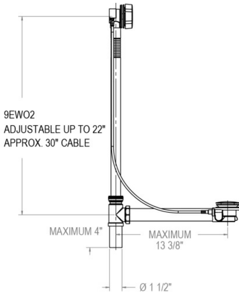
22" ADJUSTABLE CABLE DRIVEN TUBULAR WASTE & OVERFLOW (SOLID BRASS)
