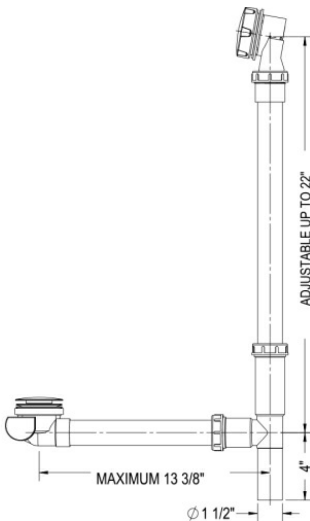
22" ADJUSTABLE CABLE DRIVEN TUBULAR WASTE & OVERFLOW (PVC WITH BRASS TRIM ONLY)
