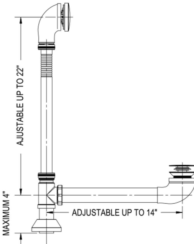
22" EXPOSED ADJUSTABLE PUSH-UP TUBULAR WASTE & OVERFLOW (SOLID BRASS)
