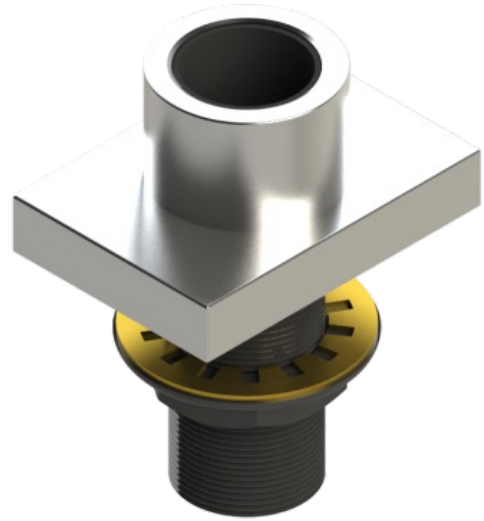
HOSE GUIDE COMPLETE WITH ROUGH-IN
