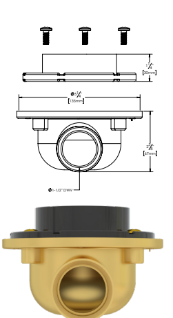
40 1.5" Brass Side Discharge
