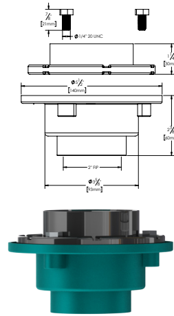
52 2" Cast Iron Straight
